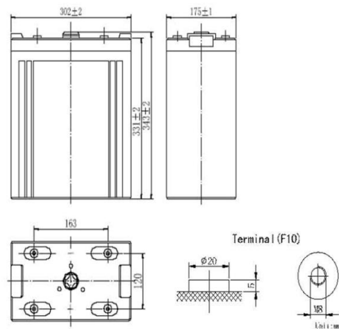
Total height with removable cover:367
